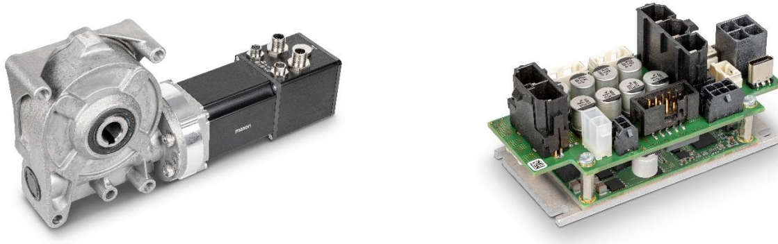
Figure: On the left is the IDX 56 with the GB12 gearhead from Parvalux. On the right is a servo controller with the new ESCON2 Module Compact 60/30.
